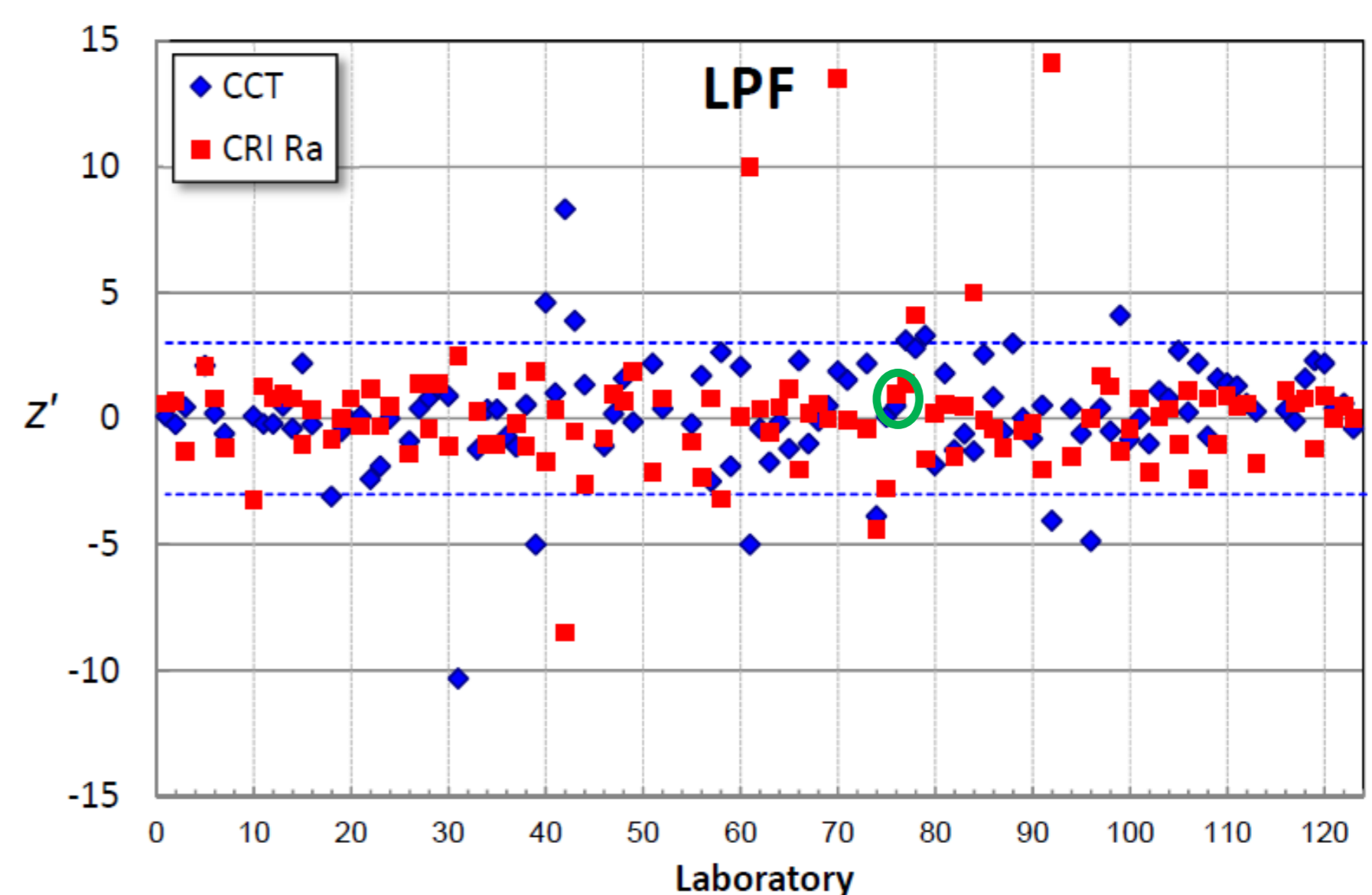
Figure 9-80. z' scores for CCT and CRI Ra for LPF
