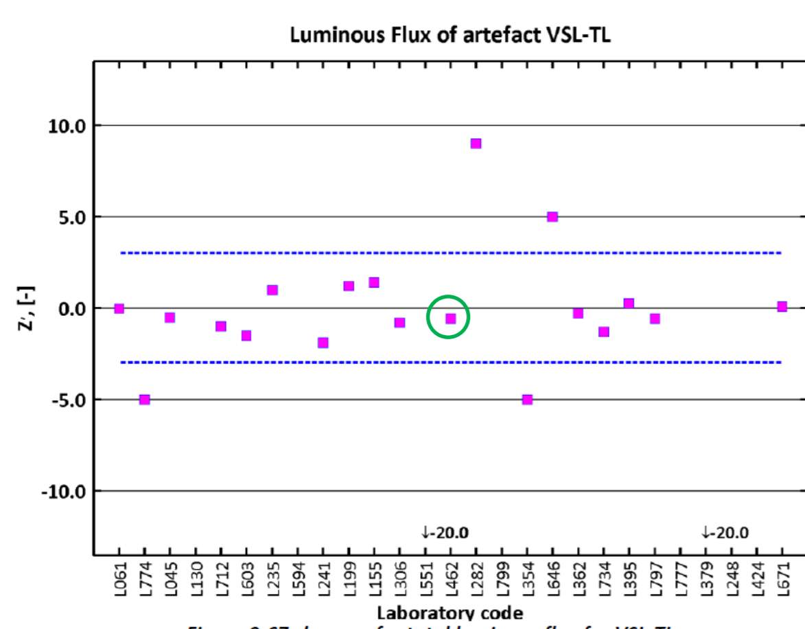
Figure 9-67 z' scores for total luminous flux for VSL-TL.
