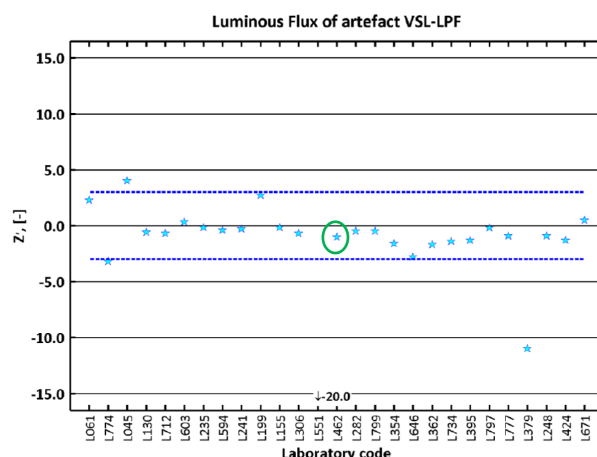
Figure 9-68 z' scores for total luminous flux for VSL-LPF.
