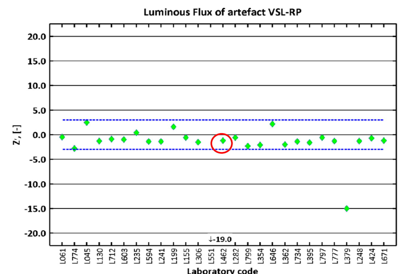
Figure 9-65 z' scores for total luminous flux for VSL-RP.
